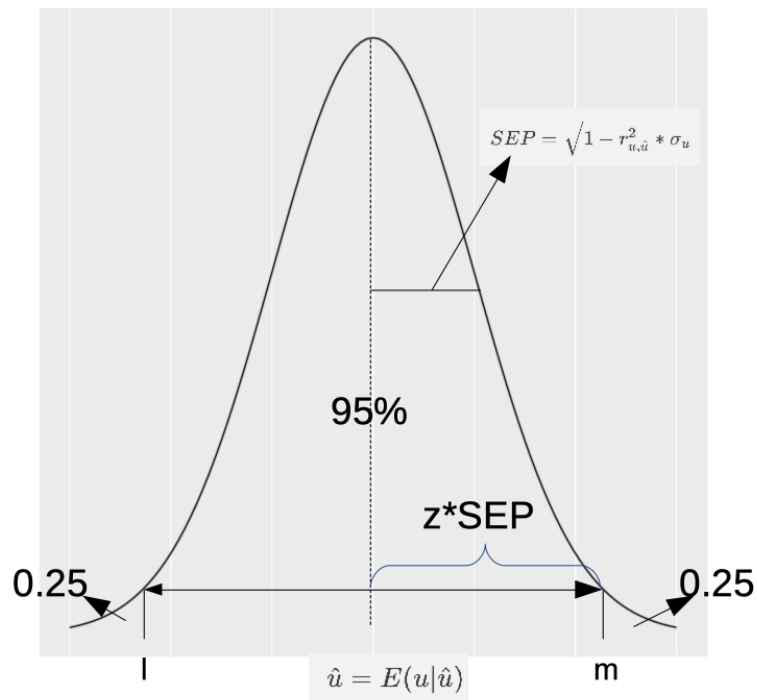
Figure 6.1: Conditional Density with Confidence Interval
