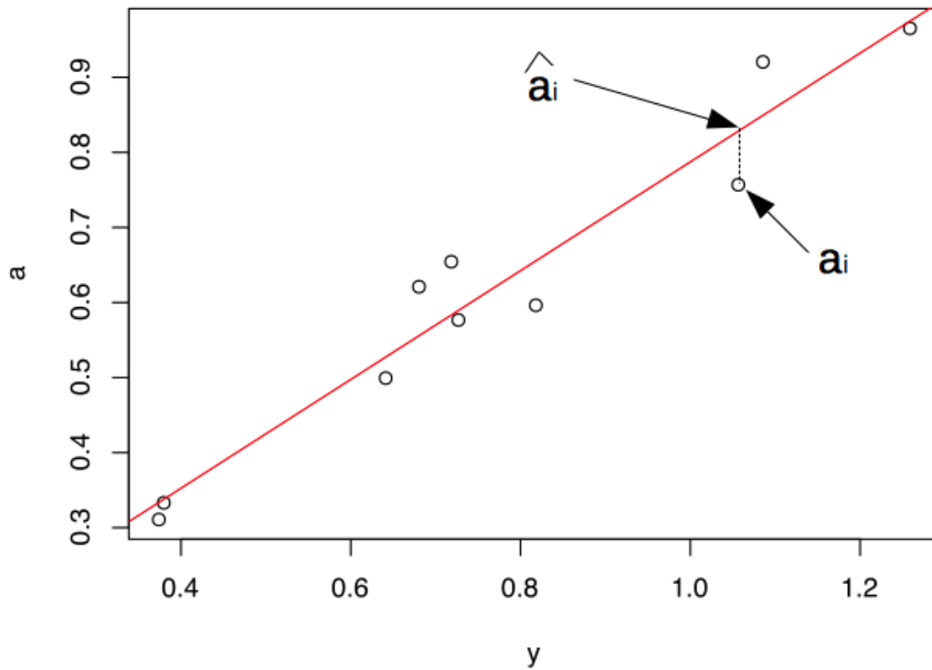
Figure 3.2: Regression of Breeding Values onto Phenotypic Observations
